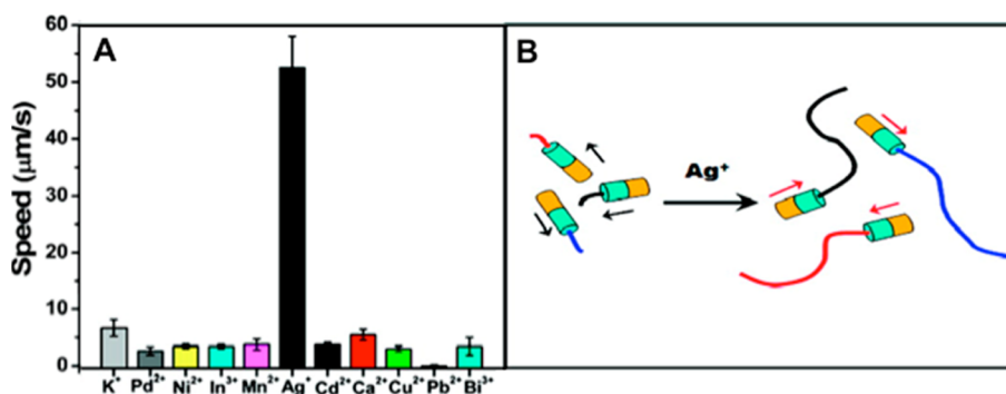
Figure 1. Motion-based sensing of trace silver ions using catalytic Au–Pt nanowire motors. (A) Selectivity: bar graph comparing the nanomotor speed in 11 different 100 \mu\text{M} metal–nitrate salt solutions (of \text{K}^+ , \text{Pd}^{2+} , \text{Ni}^{2+} , \text{In}^{3+} , \text{Mn}^{2+} , \text{Ag}^+ , \text{Cd}^{2+} , \text{Ca}^{2+} , \text{Cu}^{2+} , \text{Pb}^{2+} , and \text{Bi}^{3+} ). (B) Accelerated propulsion of catalytic nanomotors in the presence of silver ions. Reprinted from ref 61. Copyright 2009 American Chemical Society.
