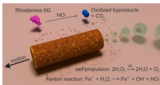
Figure 6. Tubular Fe/Pt bilayer microengines for destroying organic contaminants based on the Fenton reaction. The micromotors contain double functionality with an inner Pt layer for the self-propulsion and the outer Fe for the in situ generation of \text{Fe}^{2+} ions. The ions, along with the \text{H}_2\text{O}_2 fuel, generate \text{HO}\cdot radicals that degrade organic pollutants. Reprinted from ref 54. Copyright 2013 American Chemical Society.
